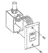
Fig. 2 - SD-TRM4 Installation Diagram
