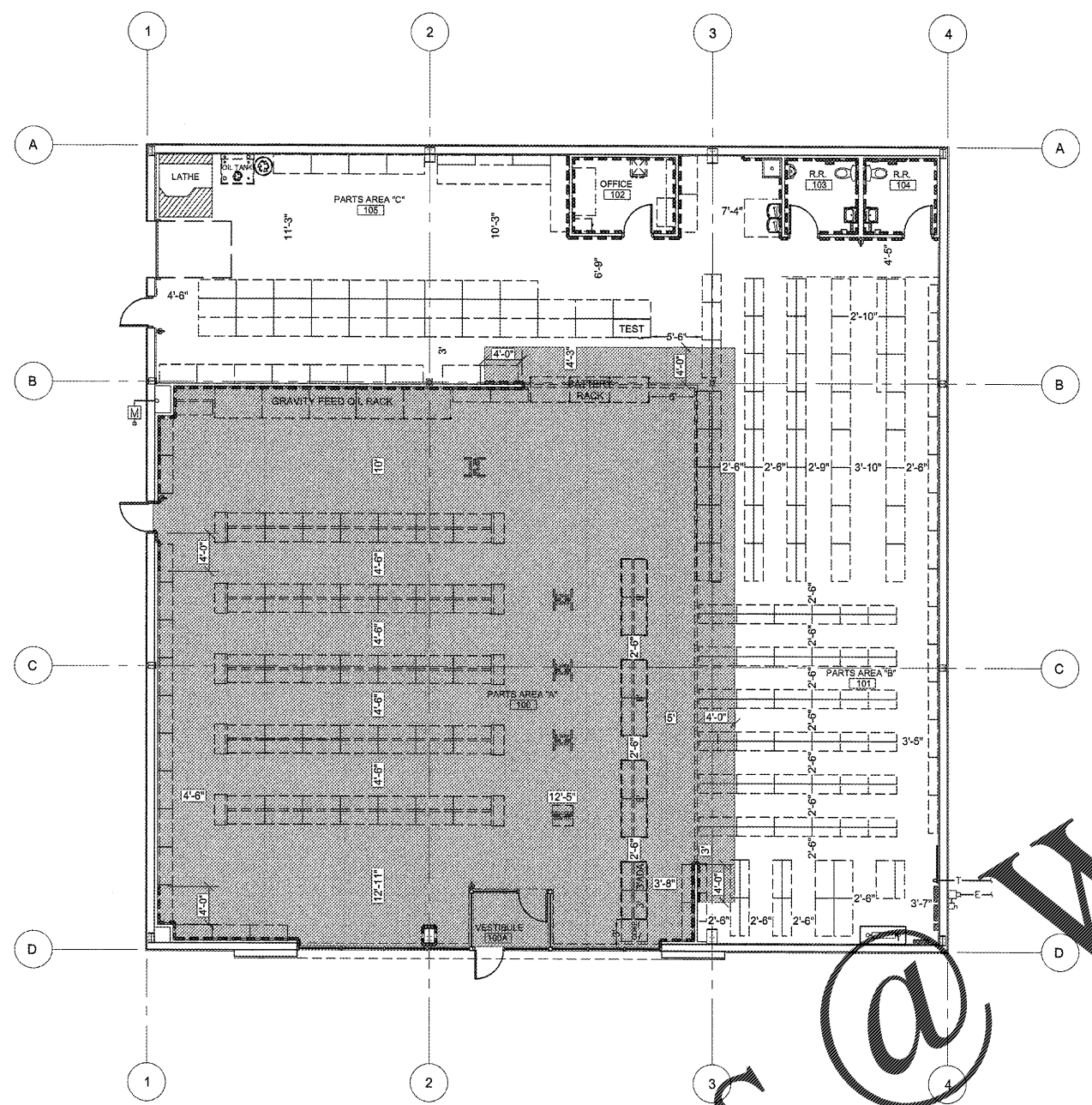
1 INTERIOR FINISH PLAN A1.2 SCALE: 1/8" = 1'-0"
