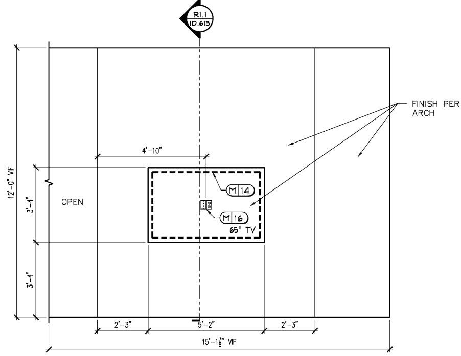
R1.1 PORCH ID.613 SCALE: 1/2" = 1'-0" NOTE: TRIM/ FINISHES PER ARCH.
