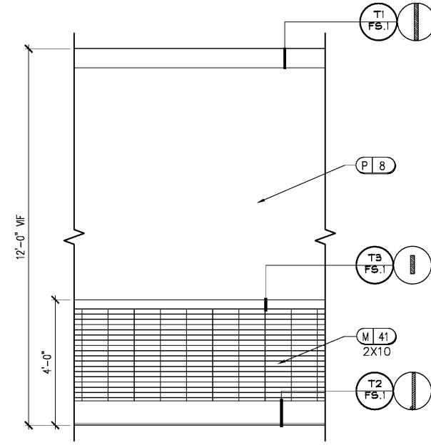
02 CYCLE/ YOGA TYP ID.612 SCALE: 1/2" = 1'-0" NOTE: 1. ALL TRIM TO BE PAINTED P5. 2. USE GREY OUTLET COVERS M57 WHERE NEEDED.
