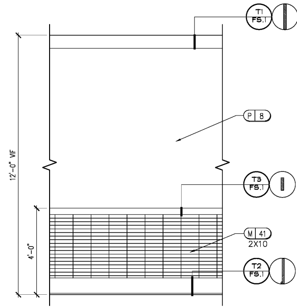
01 FREE WEIGHTS TYP ID.612 SCALE: 1/2" = 1'-0" NOTE: 1. ALL TRIM TO BE PAINTED P5. 2. USE GREY OUTLET COVERS M57 WHERE NEEDED.
