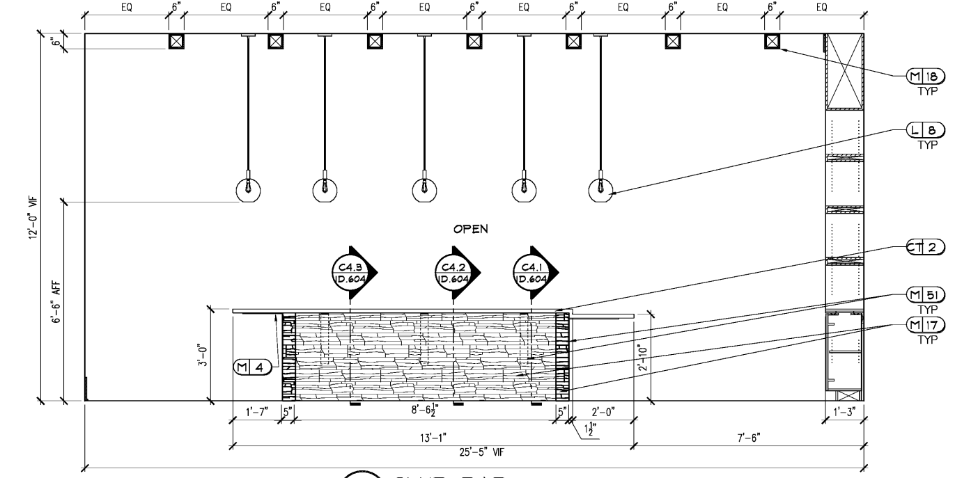
C1 CLUB BAR ID.603 SCALE: 1/2" = 1'-0" NOTE: 1. REFER TO ID.200A FOR LIGHTING LOCATIONS. 2. USE HIDDEN SUPPORT BRACKETS M4 AND M51 AS NEEDED FOR SUPPORT. 3. MITER ALL EDGES OF M18.
