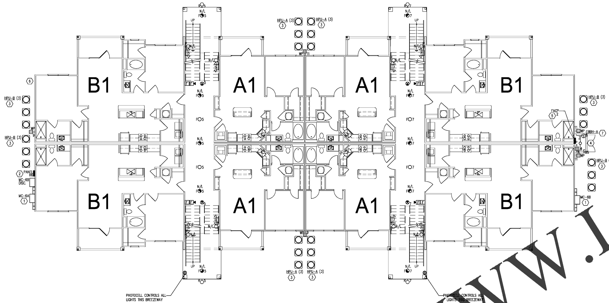
1 BUILDING 6 GROUND LEVEL - ELECTRICAL PLANS E-9.1 SCALE: 1/8" = 1'-0"
