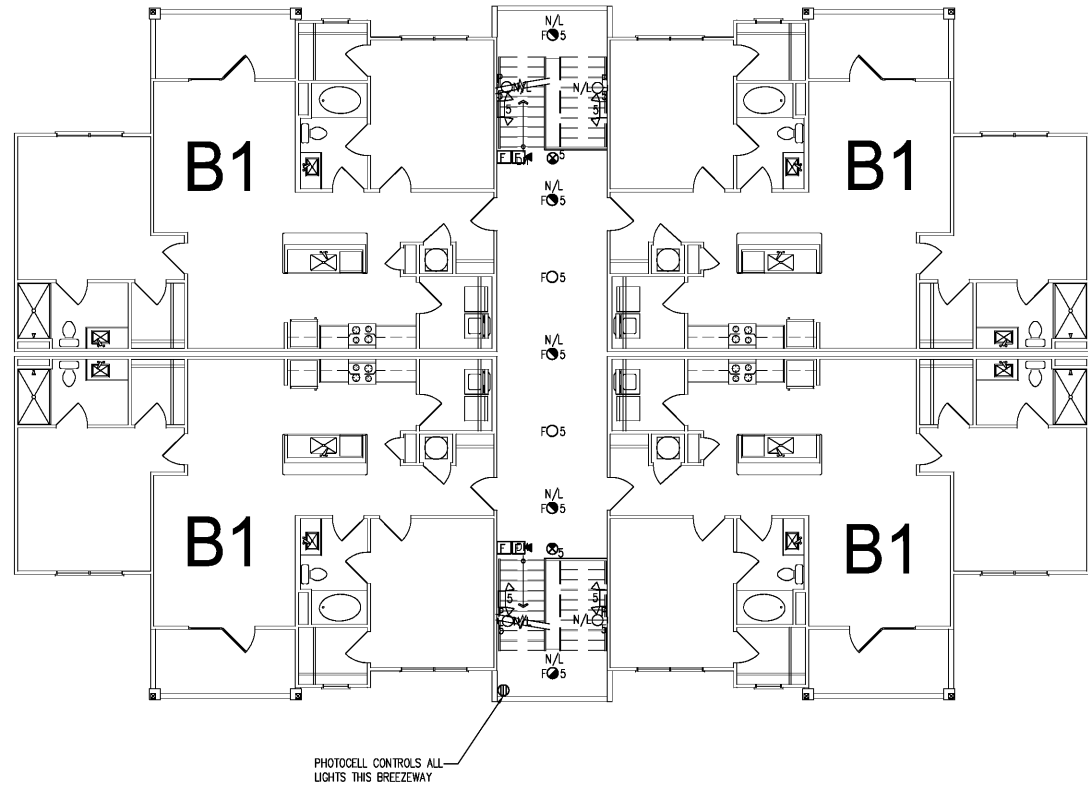
1 BUILDINGS 4 & 7 THIRD LEVEL – ELECTRICAL PLANS E-7.2 SCALE: 1/8" = 1'-0"
