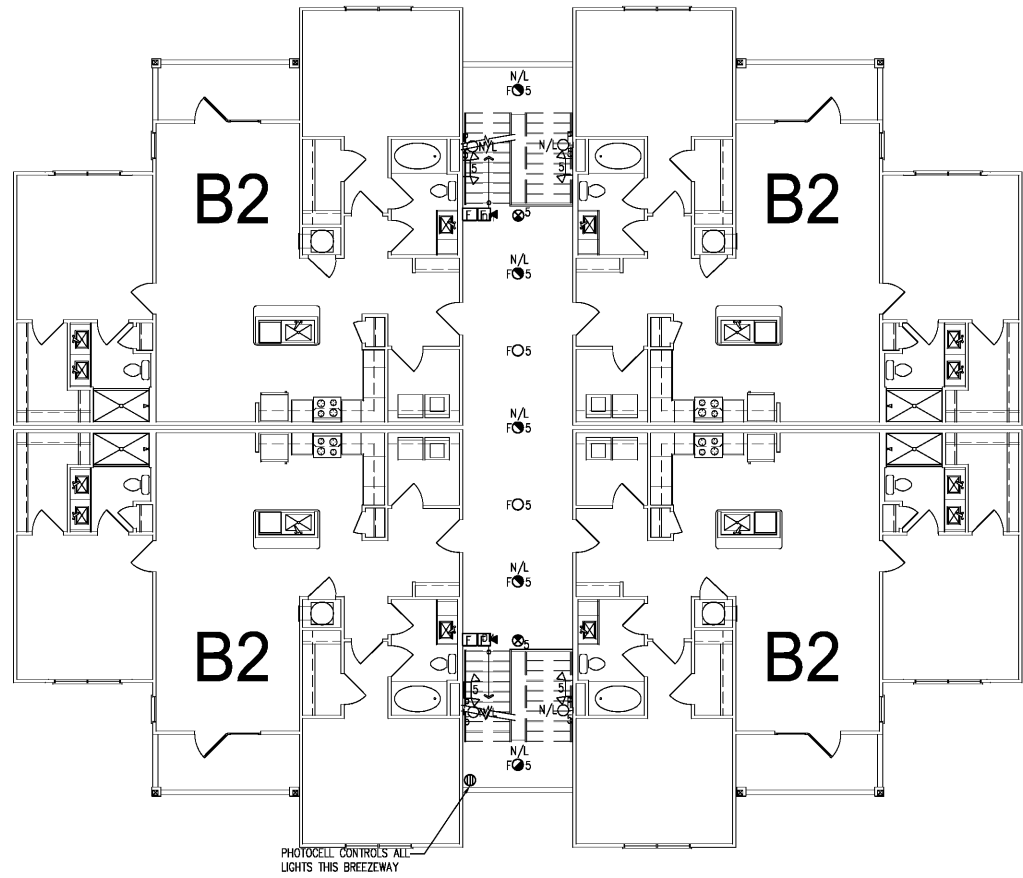
1 BUILDINGS 2 & 9 THIRD LEVEL - ELECTRICAL PLANS E-5.2 SCALE: 1/8" = 1'-0"
