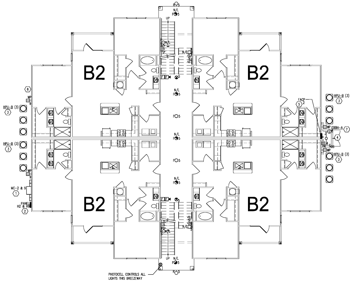
1 BUILDINGS 2 & 9 GROUND LEVEL - ELECTRICAL PLANS E-5.1 SCALE: 1/8" = 1'-0"
