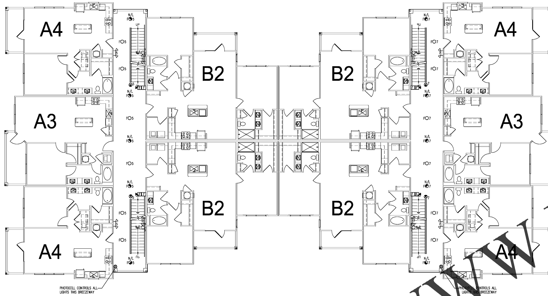
1 BUILDING 1 SECOND LEVEL - ELECTRICAL PLANS E-4.2 SCALE: 1/8" = 1'-0"
