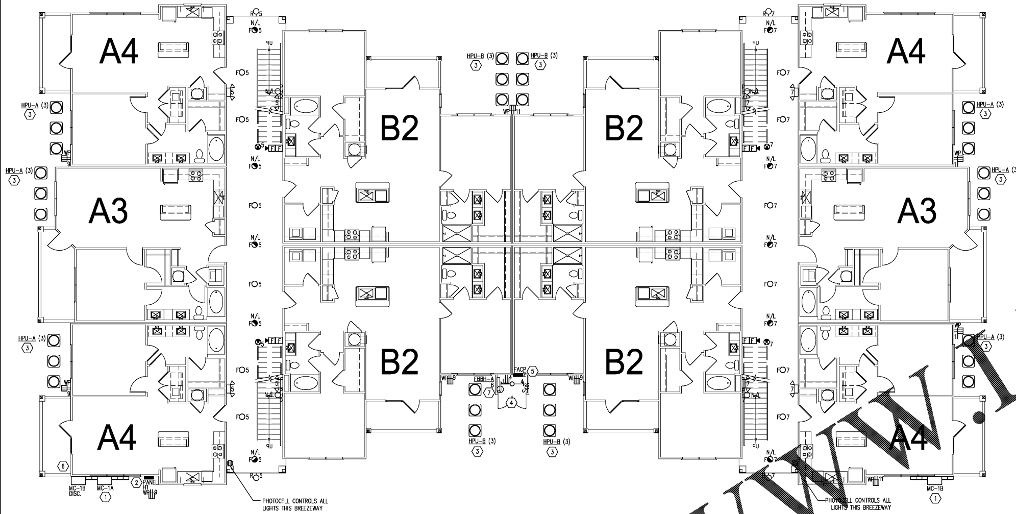
1 BUILDING 1 GROUND LEVEL - ELECTRICAL PLANS E-4.1 SCALE: 1/8" = 1'-0"
