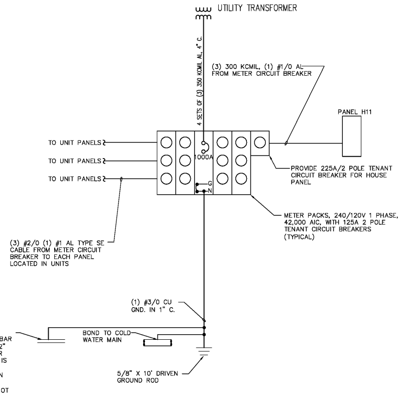
1 ELECTRICAL RISER DIAGRAM - BLDG. 11A E-16.9 NOT TO SCALE
