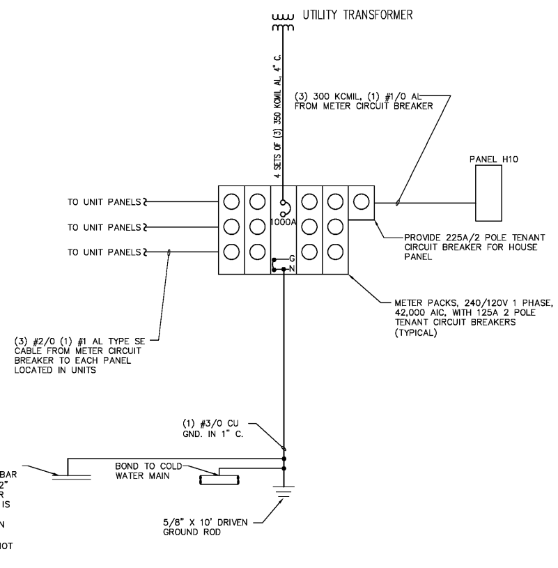
1 ELECTRICAL RISER DIAGRAM - BLDG. 10A E-16.8 NOT TO SCALE
