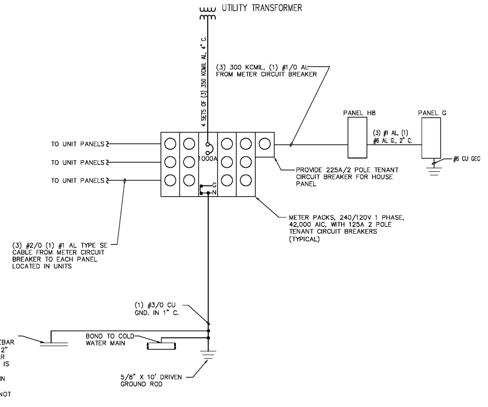
1 ELECTRICAL RISER DIAGRAM - BLDG. 8A E-16.7 NOT TO SCALE
