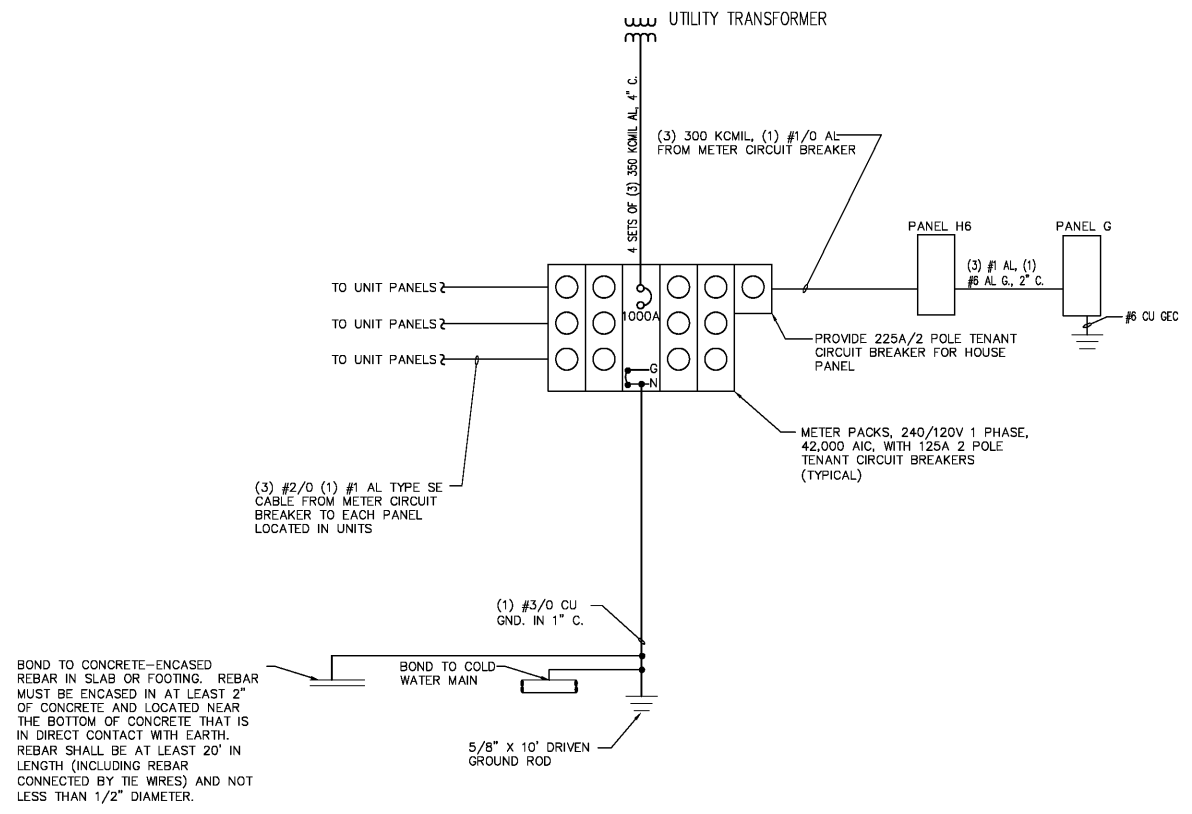
1 ELECTRICAL RISER DIAGRAM - BLDG. 6A E-16.6 NOT TO SCALE
