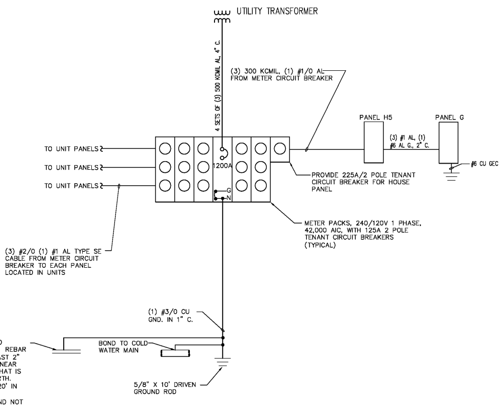
1 ELECTRICAL RISER DIAGRAM - BLDG. 5A E-16.5 NOT TO SCALE
