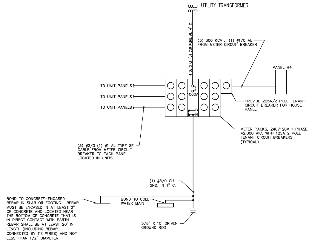
1 ELECTRICAL RISER DIAGRAM - BLDG. 4 E-16.4 NOT TO SCALE
