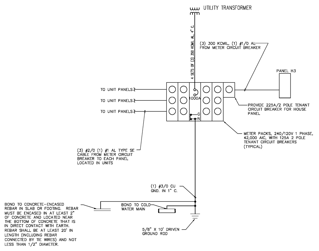
1 ELECTRICAL RISER DIAGRAM - BLDG. 3A E-16.3 NOT TO SCALE
