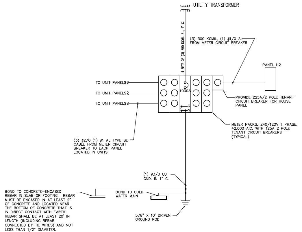
1 ELECTRICAL RISER DIAGRAM - BLDG. 2 E-16.2 NOT TO SCALE
