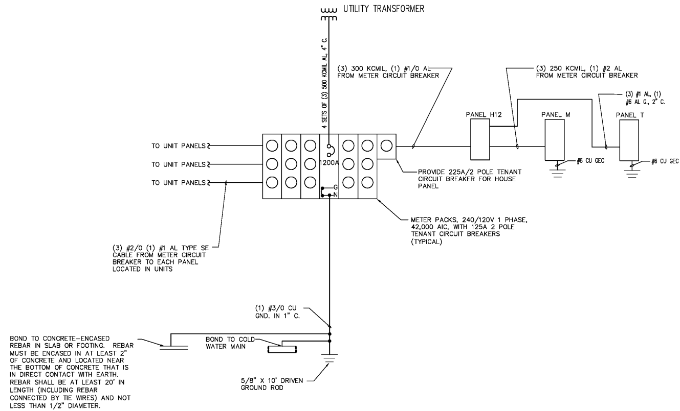
1 ELECTRICAL RISER DIAGRAM - BLDG. 12A E-16.10 NOT TO SCALE
