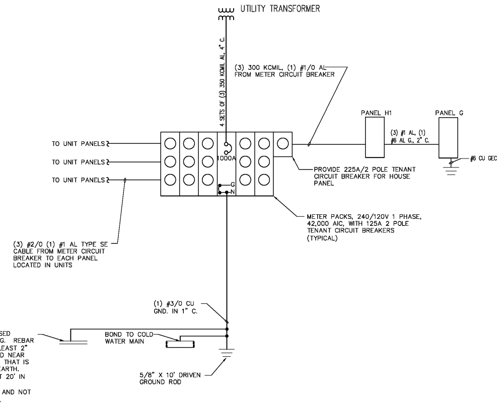
1 ELECTRICAL RISER DIAGRAM - BLDG. 1A E-16.1 NOT TO SCALE
