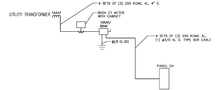
3 ELECTRICAL RISER DIAGRAM - LEASING OFFICE E-16.1 NOT TO SCALE
