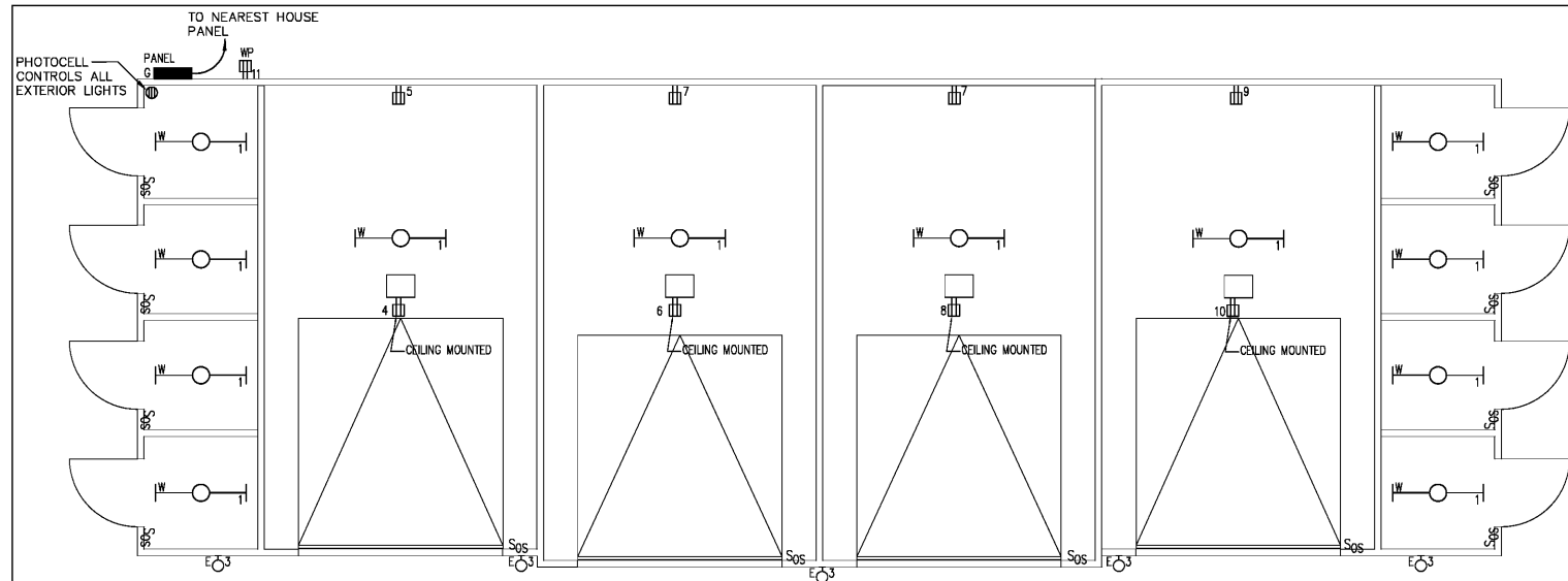
1 4 BAY GARAGE WITH STORAGE - ELECTRICAL PLAN E-14.1 SCALE: 1/4" = 1'-0"
