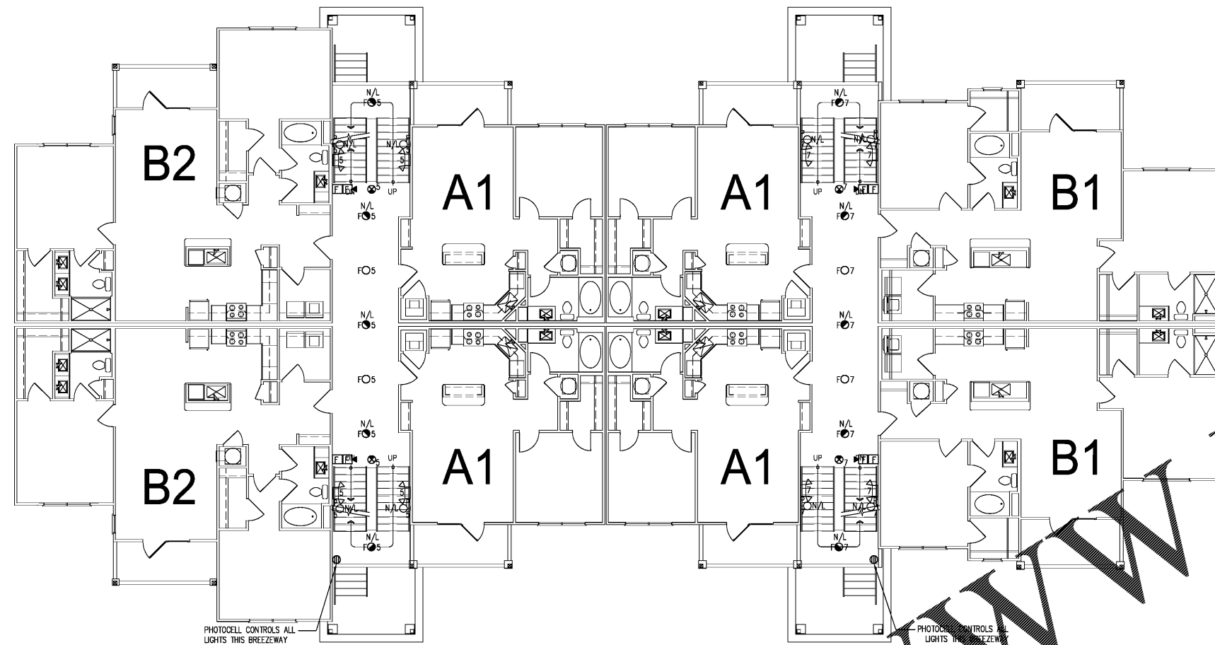
1 BUILDING 11 SECOND LEVEL - ELECTRICAL PLANS E-12.2 SCALE: 1/8" = 1'-0"
