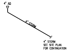
3 MAINTENANCE STORM RISER P-9 NOT TO SCALE
