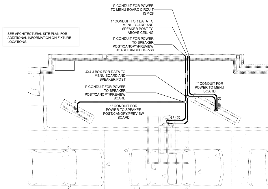
2 ENLARGED ELECTRICAL DRIVE-THRU SITE PLAN B 1/4" = 1'-0" NORTH
