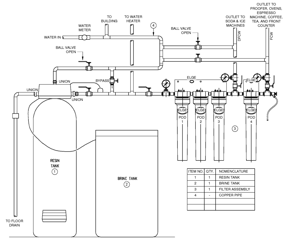
6 WATER FILTER SYSTEM DETAIL SCALE: NTS
