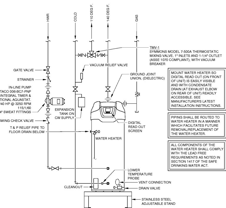
1 WATER HEATER DETAIL SCALE: NTS
