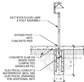
1 | LAMP BASE @ CONCRETE PATIO 1/2" = 1'-0"
