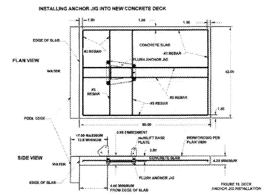
S. R. SMITH multiLIFT INSTALLING ANCHOR JIG INTO NEW CONCRETE DECK
