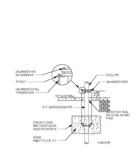
1 FIRE PROTECTION FOUNDATION WALL SERVICE ENTRY SCHEMATIC NOT TO SCALE
