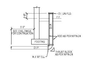
3 FIRE SERVICE ENTRANCE DETAIL 1" = 10'-0"
