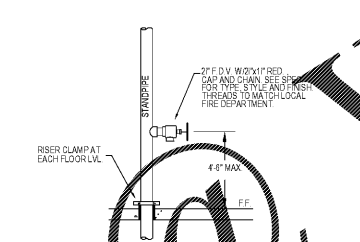
6 INTERMEDIATE LEVEL FIRE DEPARTMENT VALVE DETAIL 1" = 10'-0"
