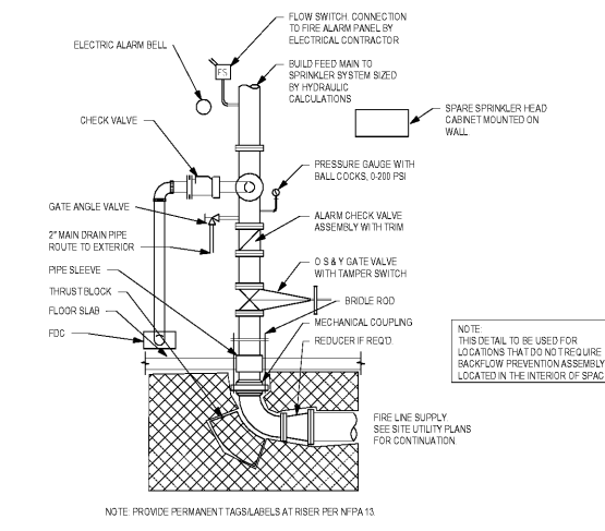
2 FIRE RISER DETAIL NOT TO SCALE
