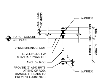
2 TYP. ANCHOR ROD DETAIL SCALE: NTS
