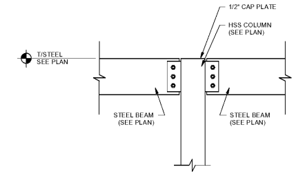
3 TYP. BEAM TO COLUMN CONNECTION SCALE: NTS
