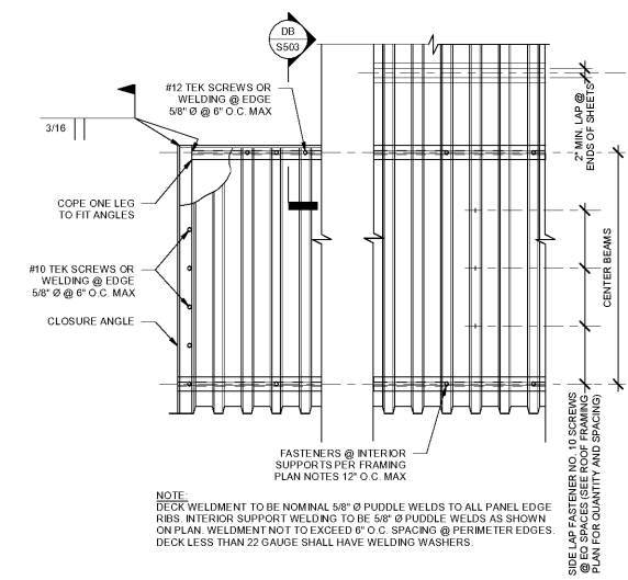
5 TYP. METAL DECK ATTACHMENT DETAIL SCALE: NTS
