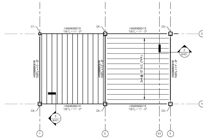
2 PLAN @ TRELLIS S401 SCALE: 1/4" = 1'-0"
