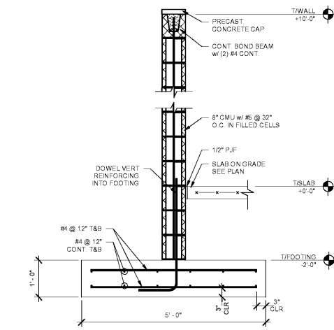
9 DUMPSTER WALL S401 SCALE: 3/4" = 1'-0"
