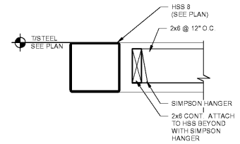
3 TRELLIS FRAMING TO STEEL BEAM S401 SCALE: 1 1/2" = 1'-0"
