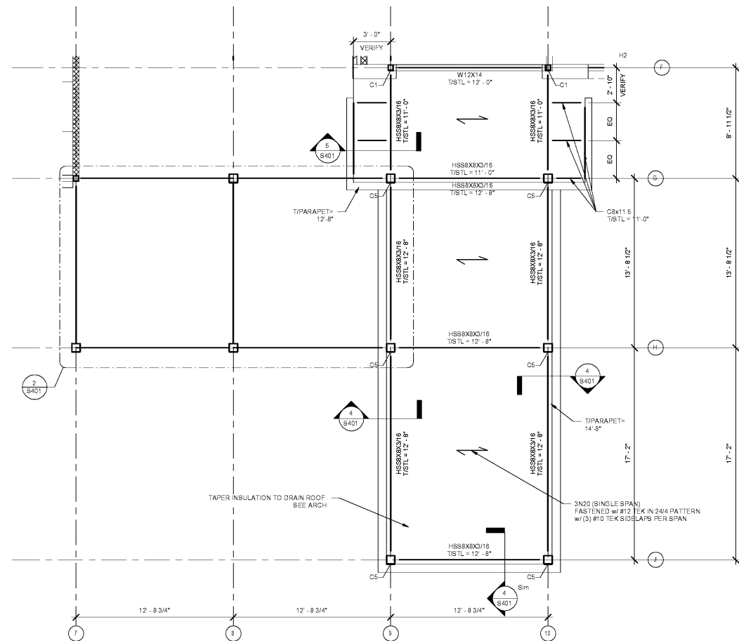
1 PLAN @ PORTE COCHERE S401 SCALE: 1/4" = 1'-0"
