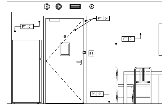
8 KING 1 BEDROOM ADA ELEVATION ID3.12 SCALE: 1/2" = 1'-0"
