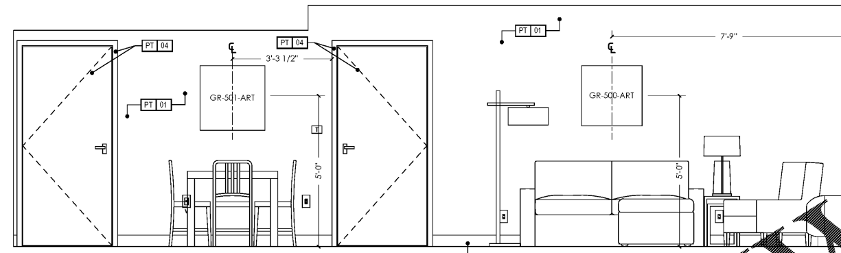
5 KING 1 BEDROOM ADA ELEVATION ID3.12 SCALE: 1/2" = 1'-0"
