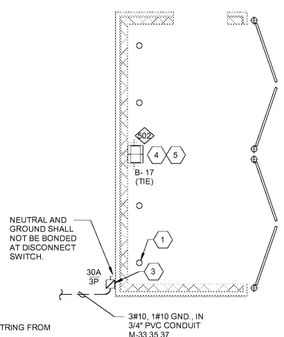
5 DISPENSOR PUMP AND INTRINSICALLY SAFE STUB-UP DETAIL N.T.S.
