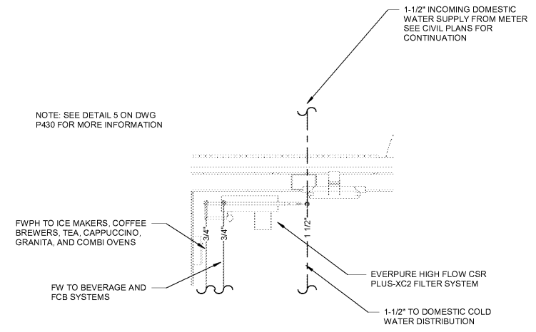
2 ENLARGED WATER PLAN 1/2" = 1'-0"
