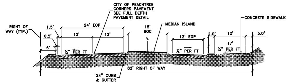
TYPICAL CROSS SECTION C-C: STA 106+25 TO 107+56 SCALE: 1"=10'
