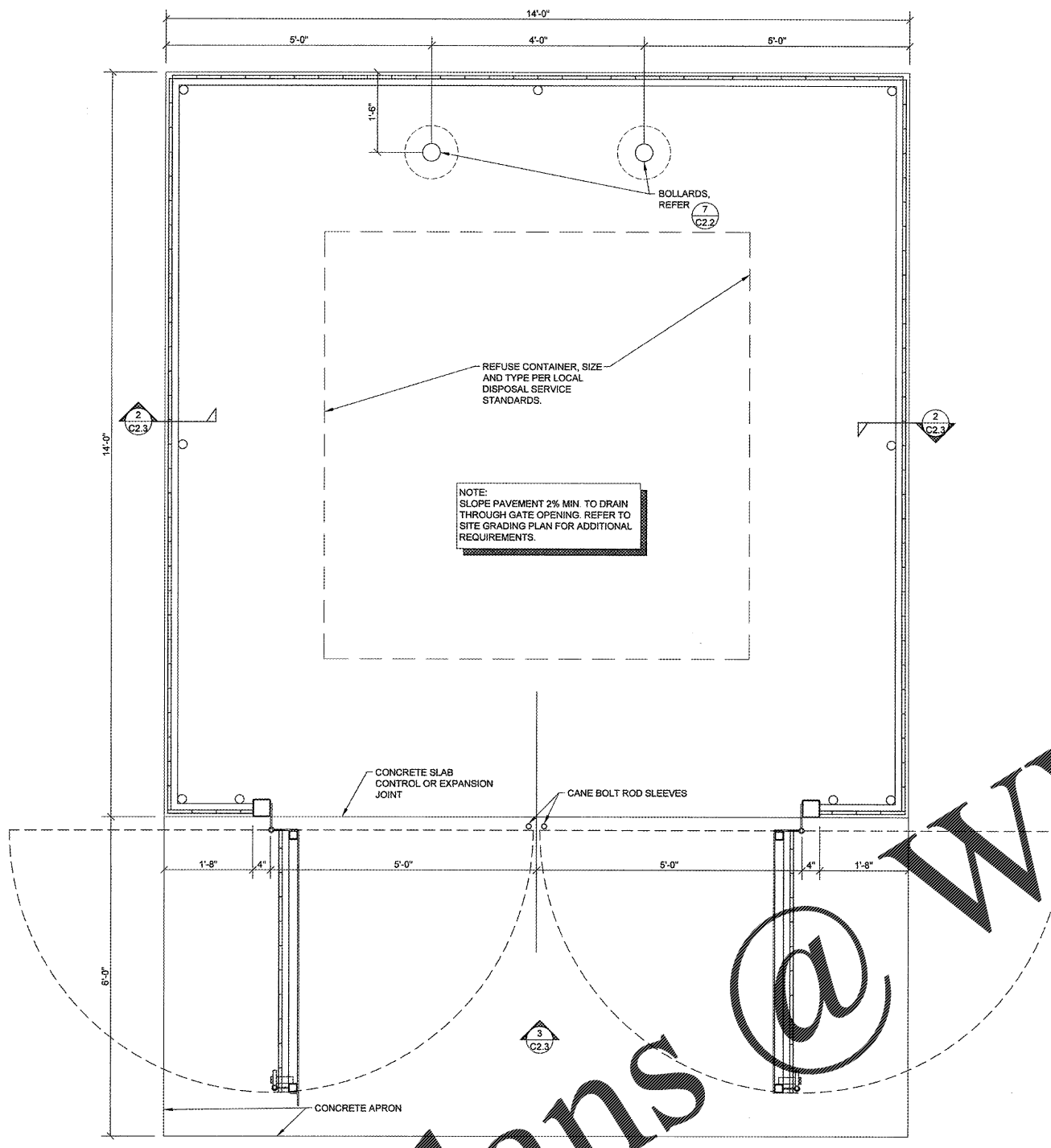
1 POLYMER COMPOSITE MATERIAL SCREEN FENCE REFUSE ENCLOSURE PLAN C2.3 SCALE: 3/4" = 1'-0"
