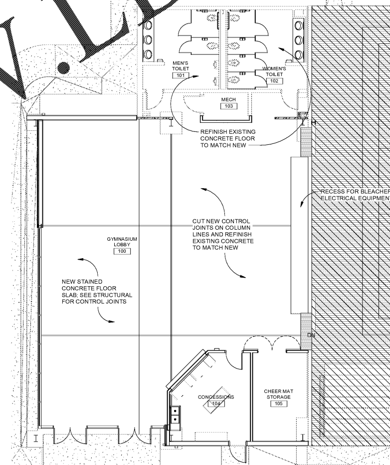
2 Gym Addition Finish Plan SCALE: 1/8" = 1'-0"
