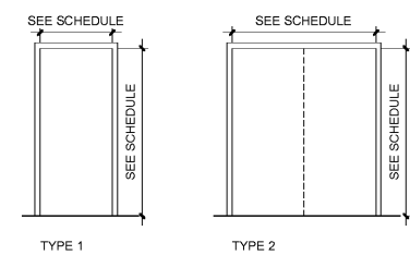
FRAME TYPES
