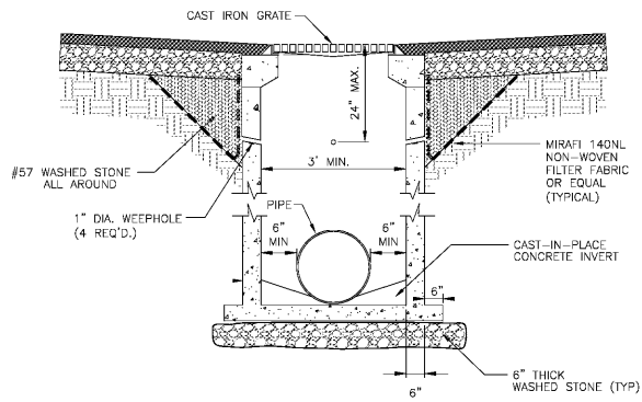
CATCH BASIN/JUNCTION BOX N.T.S.
