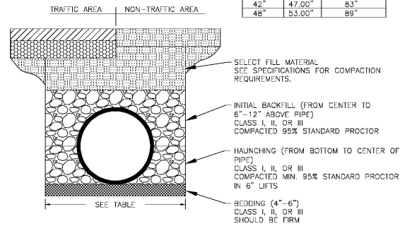
HDPE PIPE TRENCHING & BACKFILL REQUIREMENTS
