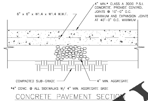
CONCRETE PAVEMENT SECTION
