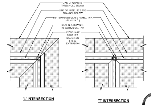
10 INT SF DTL - INTERSECTING PANELS 3" = 1'-0"
