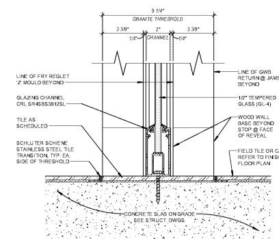
1 INT SF DTL - SILL (6\"/>
