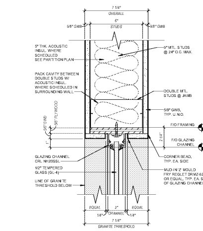
2 INT SF DTL - JAMB (6\"/>
