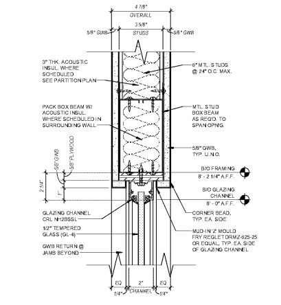
13 INT SF DTL - HEAD (3-5/8\"/>
