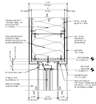
16 INT SF DTL - 451T HEAD (8\"/>
