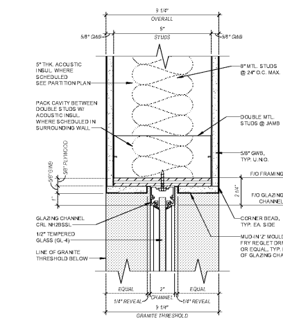
5 INT SF DTL - JAMB (8\"/>
