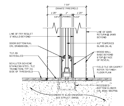
4 INT SF DTL - SILL (8\"/>
