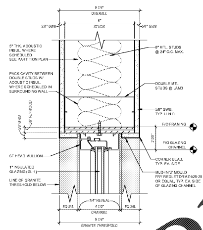
15 INT SF DTL - 451T JAMB (6\"/>
