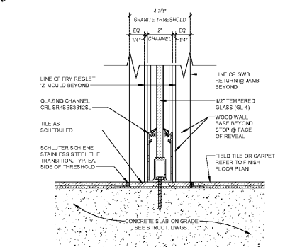
7 INT SF DTL - DOOR SILL (6\"/>
