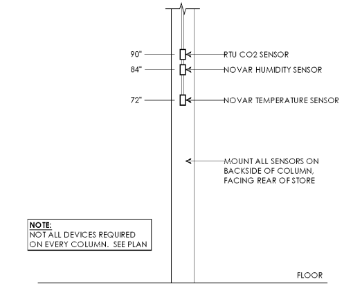
9 SENSOR MOUNTING DETAIL
