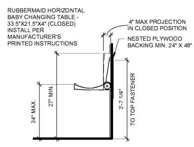
7 BABY CHANGING STATION 1/2" = 1'-0"
