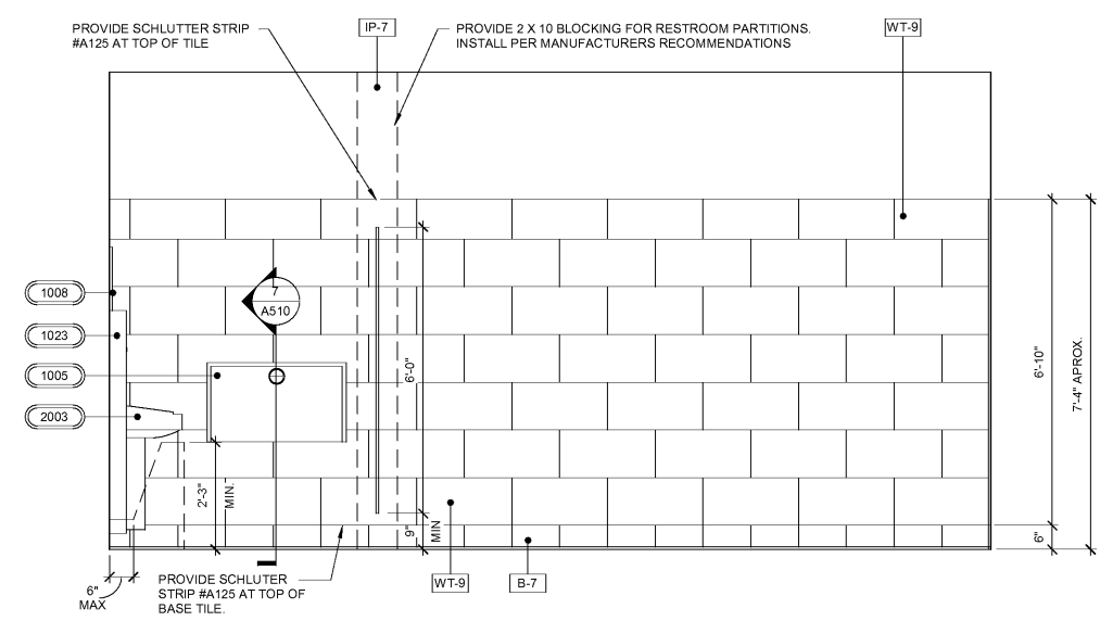
1 INTERIOR ELEVATION AT MEN'S RESTROOM 1/2" = 1'-0"
