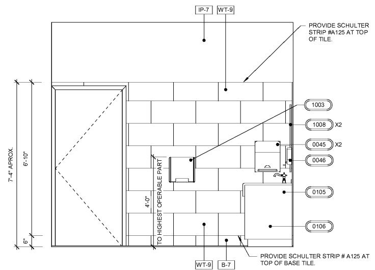
4 INTERIOR ELEVATION AT MEN'S RESTROOM 1/2" = 1'-0"
