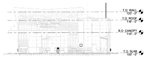
4 west elevation SCALE | 1/8" = 1'-0"
