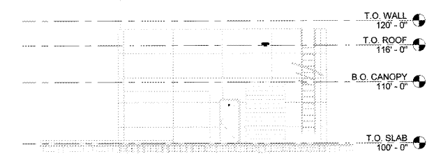
5 east elevation SCALE | 1/8" = 1'-0"
