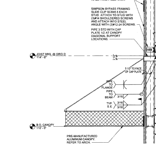
03 framing along line D SCALE | 3/4" = 1'-0"
