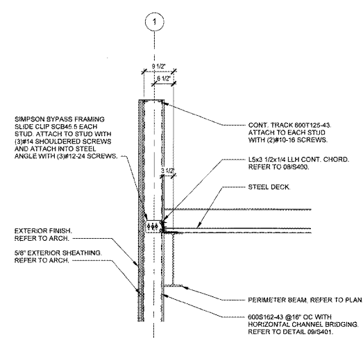
01 framing along line 1 SCALE | 3/4" = 1'-0"
