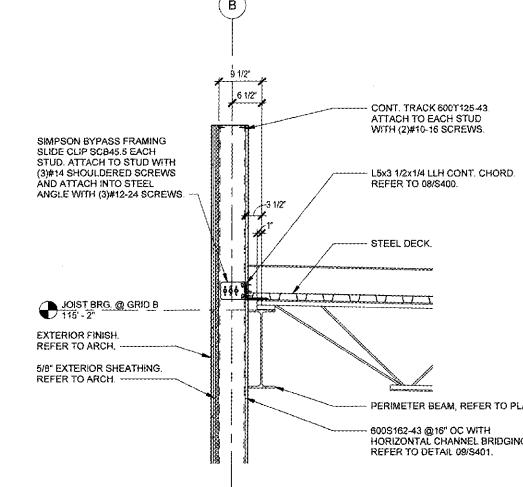
02 framing along line B SCALE | 3/4" = 1'-0"
