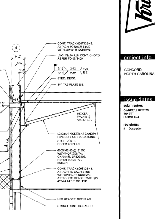
09 framing at storefront SCALE | 3/4" = 1'-0"
