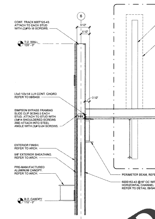
05 roof framing along line 6 SCALE | 3/4" = 1'-0"
