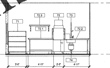
13 Elevation Dishroom Plan West SCALE | 1/4" = 1'-0"
