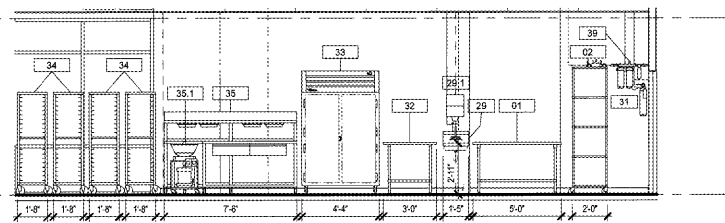
9 Elevation Production South SCALE | 1/4" = 1'-0"
