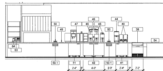
7 Elevation Bev Line SCALE | 1/4" = 1'-0"
