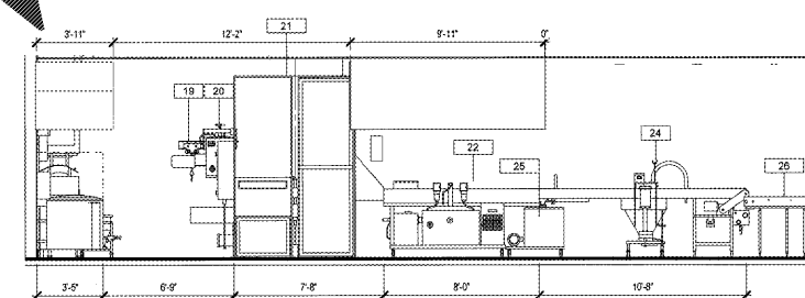
11 Elevation Production North Far SCALE | 1/4" = 1'-0"
