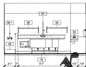
12 Elevation Dishroom Plan East SCALE | 1/4" = 1'-0"
