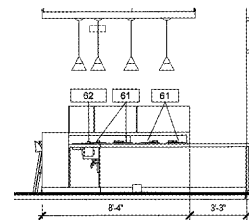
1 Elevation Mobile Pickup SCALE | 1/4" = 1'-0"
