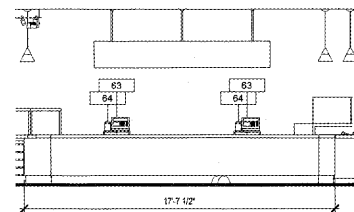
3 Elevation POS SCALE | 1/4" = 1'-0"
