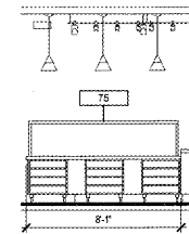
4 Elevation Doughnut Case SCALE | 1/4" = 1'-0"
