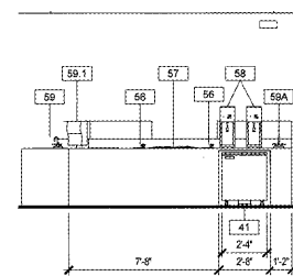
6 Elevation Shake Station SCALE | 1/4" = 1'-0"
