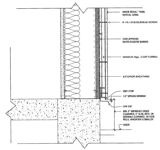
01 hardie panel @ foundation at grade SCALE | 3" = 1'-0"
