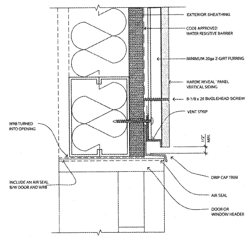
02 hardie panel @ door & window head SCALE | 3" = 1'-0"
