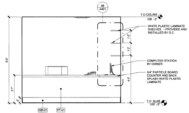
03 manager's office elevation SCALE | 1/2" = 1'-0"
