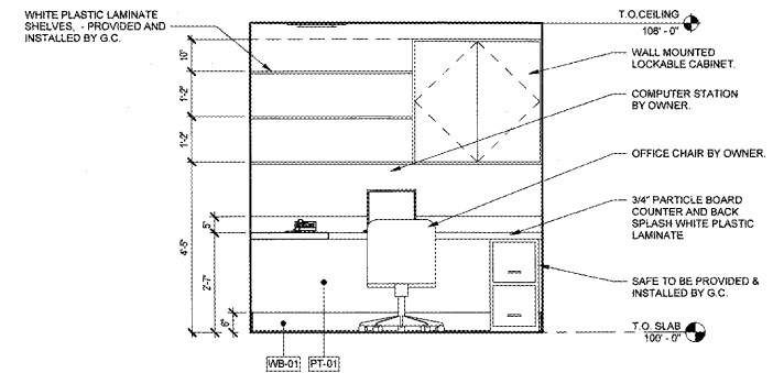
02 manager's office elevation SCALE | 1/2" = 1'-0"
