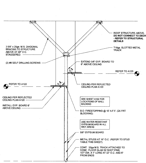
A wall type SCALE | 1/2" = 1'-0"
