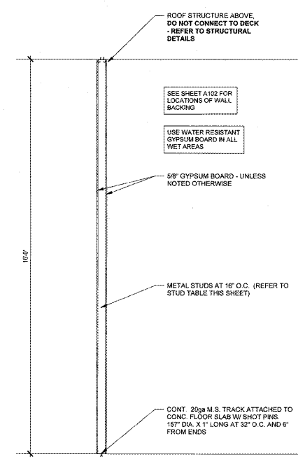
B wall type SCALE | 1/2" = 1'-0"
