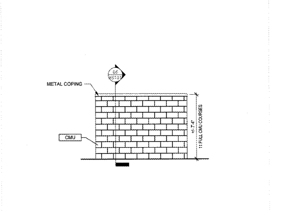
05 trash enclosure - elevation SCALE | 1/4" = 1'-0"
