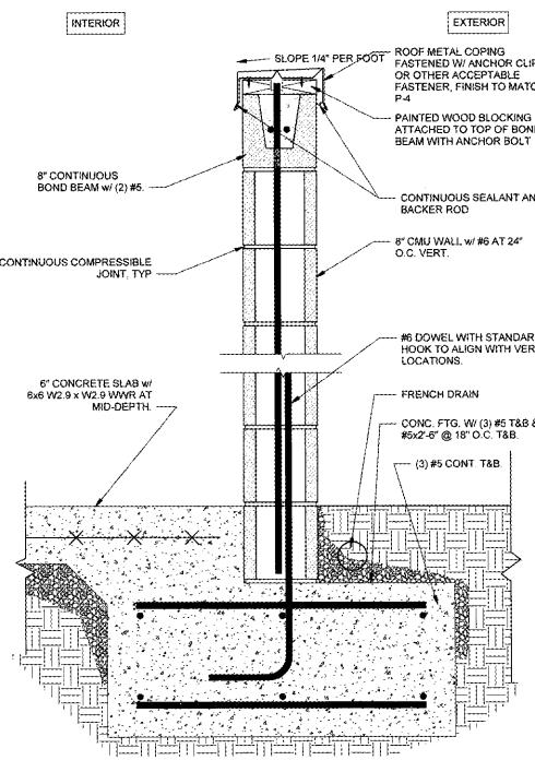
07 trash enclosure - detail SCALE | 1 1/2" = 1'-0"
