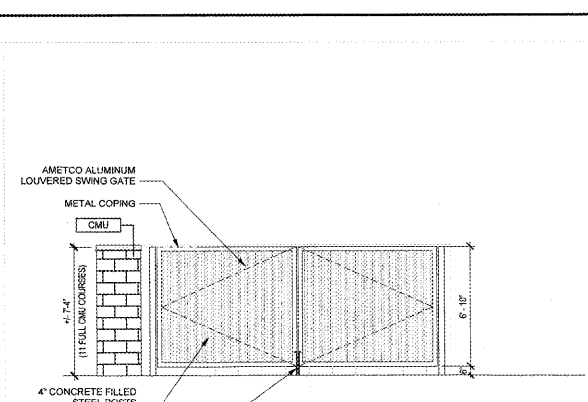
06 trash enclosure - section SCALE | 1/2" = 1'-0"
