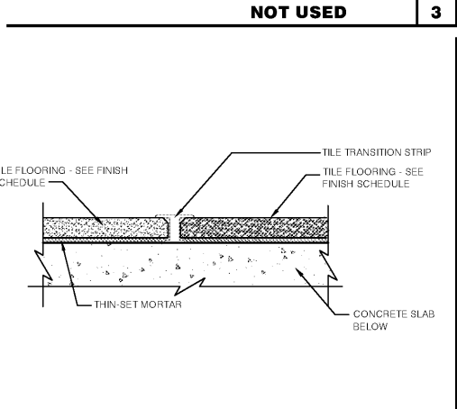
FLOOR TRANSITION 3'-1'-0" 2
