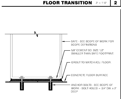
SAFE PEDESTAL 1-1/2'-1'-0" 1
