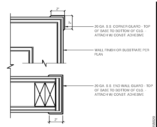
CORNER GUARD 3'-1'-0" 15
